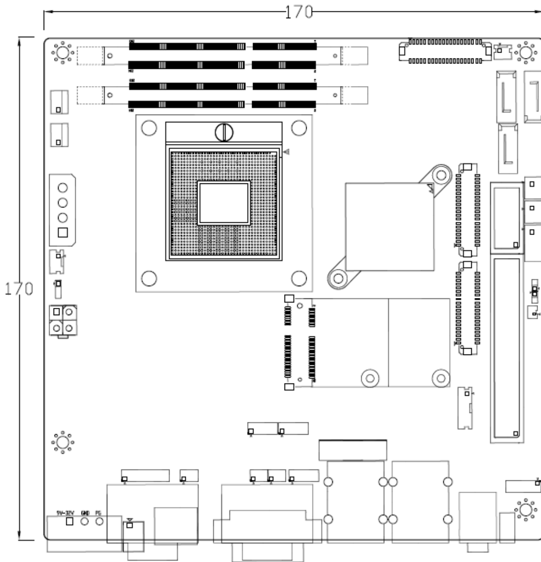
Figure 2.1: Mainboard Dimensions
